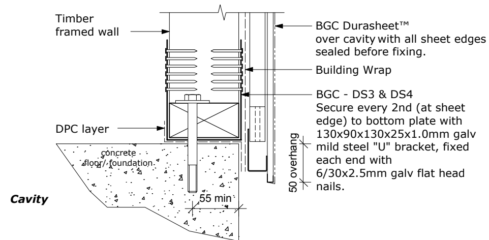
Brace Element Hold Down - Construction Detail BGC - DS3 & DS4 Sheet overhang & Bracket (concrete floor)
