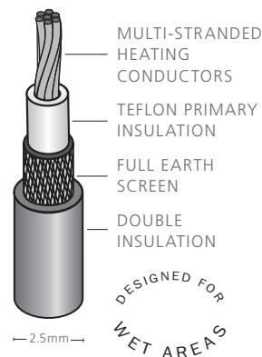
Wire cross-section
