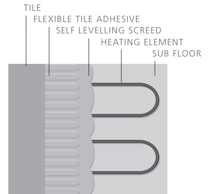
Installation diagram
