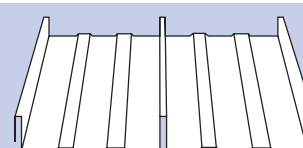
DECKING Width: 430mm Cover: 406mm Height: 45mm
