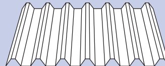
BB900 Width: 1000mm Cover: 885mm Height: 36mm
