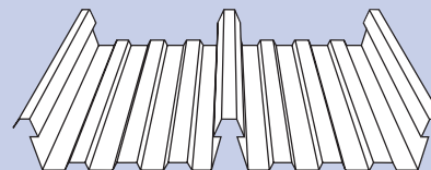
HI RIB Width: 525mm Cover: 500mm Height: 50mm
