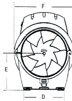
Dimensions - MF
