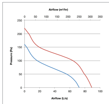
Performance - MF125
