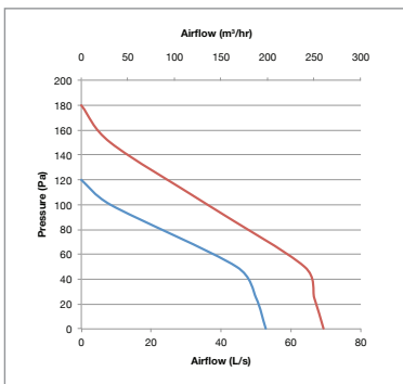
Performance - MF100
