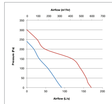
Performance - MF150
