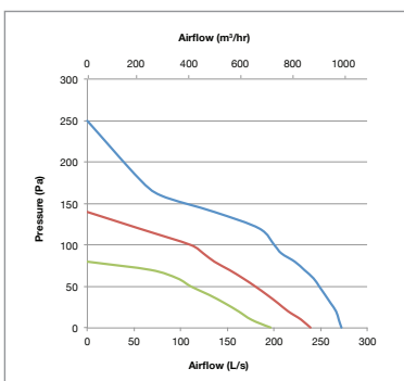
Performance - MF100
