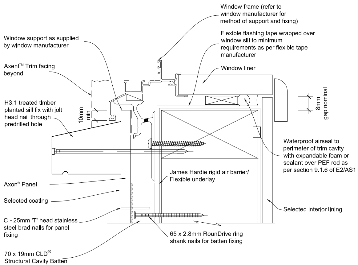
Figure 29: Window sill with planted sill
