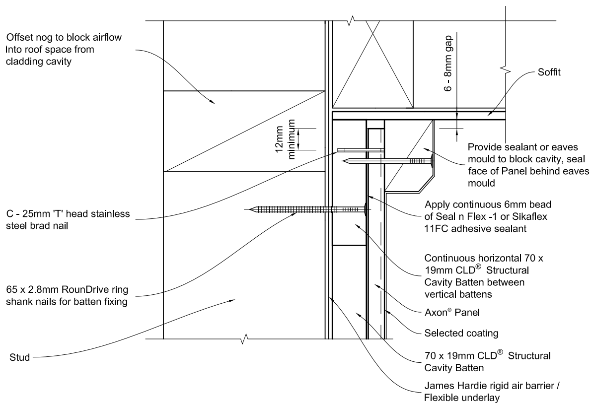
Figure 32: Soffit detail
