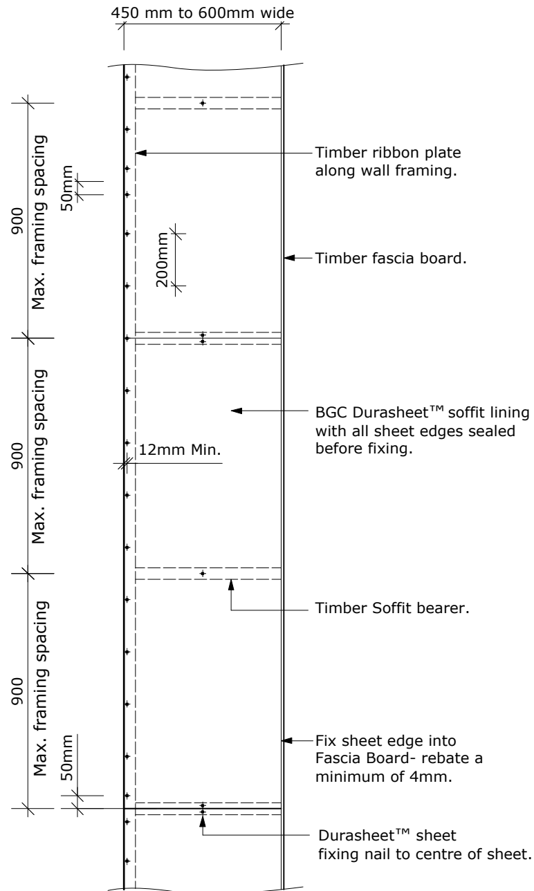
BGC Durasheet™ 450mm to 600mm Wide Soffit & Eaves Setout
