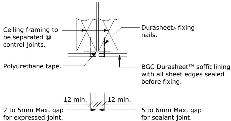
Timber Frame - Control Joint Detail
