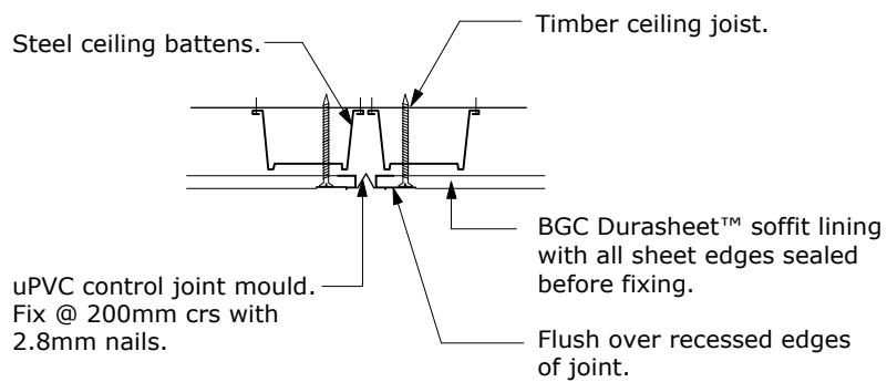
Metal Frame - Control Joint Detail
