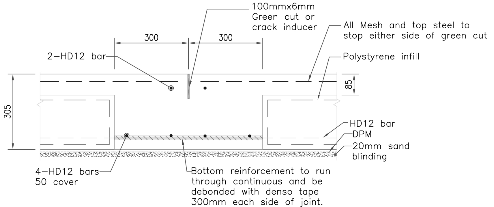
Free Joint Detail
