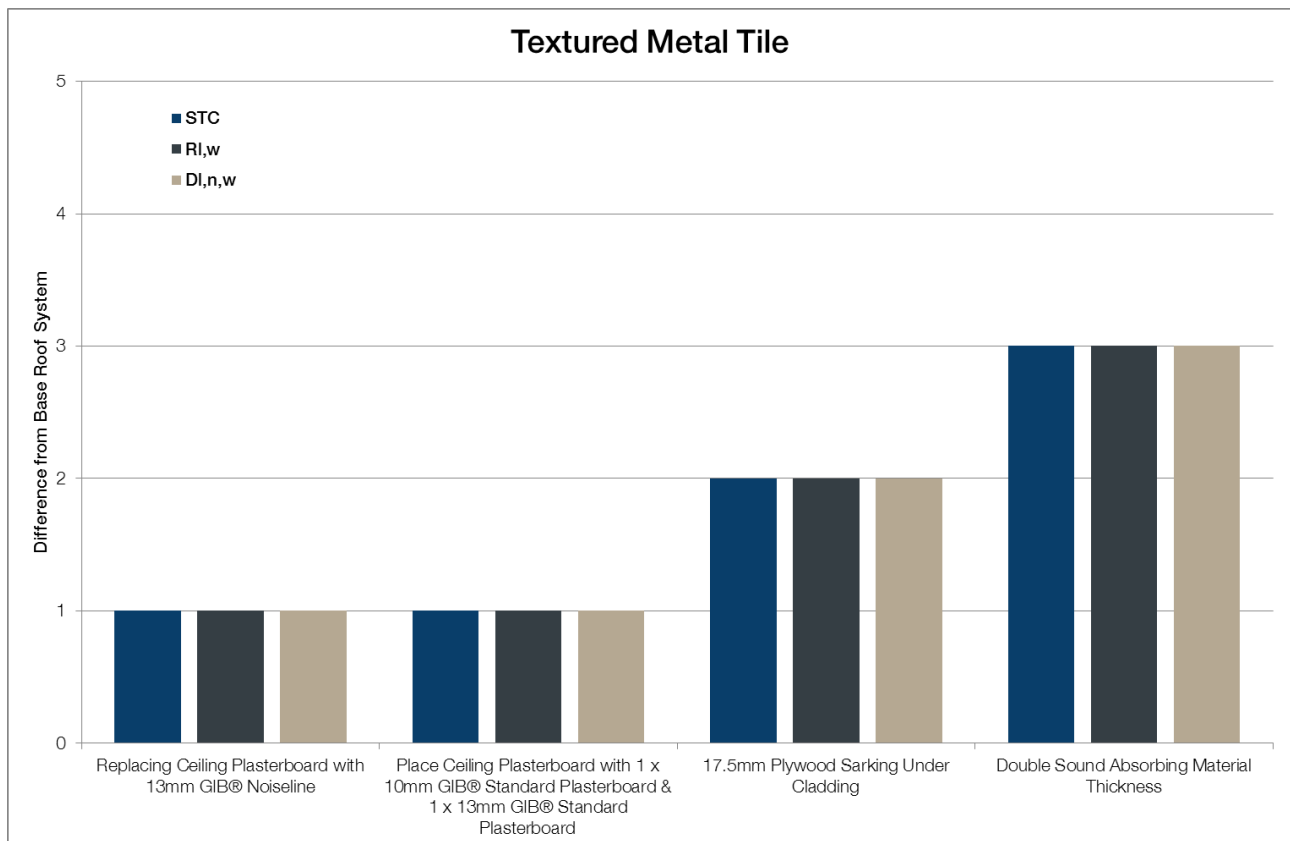
Figure 1 - Differences from Base System for Textured Metal Tile
