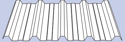
METCOM Width: 1022mm Cover: 930mm Height: 45mm
