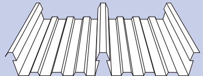
HI RIB Width: 525mm Cover: 500mm Height: 50mm
