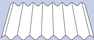
SUPER SIX Width: 1104mm Cover: 1000mm Height: 45mm
