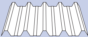
MULTISPAN/RIBSPAN Width: 990mm Cover: 900mm Height: 60mm
