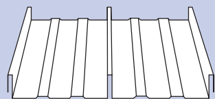
DECKING Width: 430mm Cover: 406mm Height: 45mm
