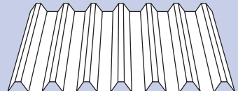
BB900 Width: 1000mm Cover: 885mm Height: 36mm
