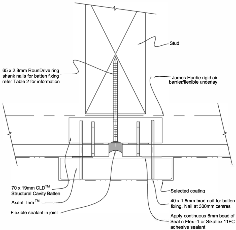
Figure 40: External corner with facings
