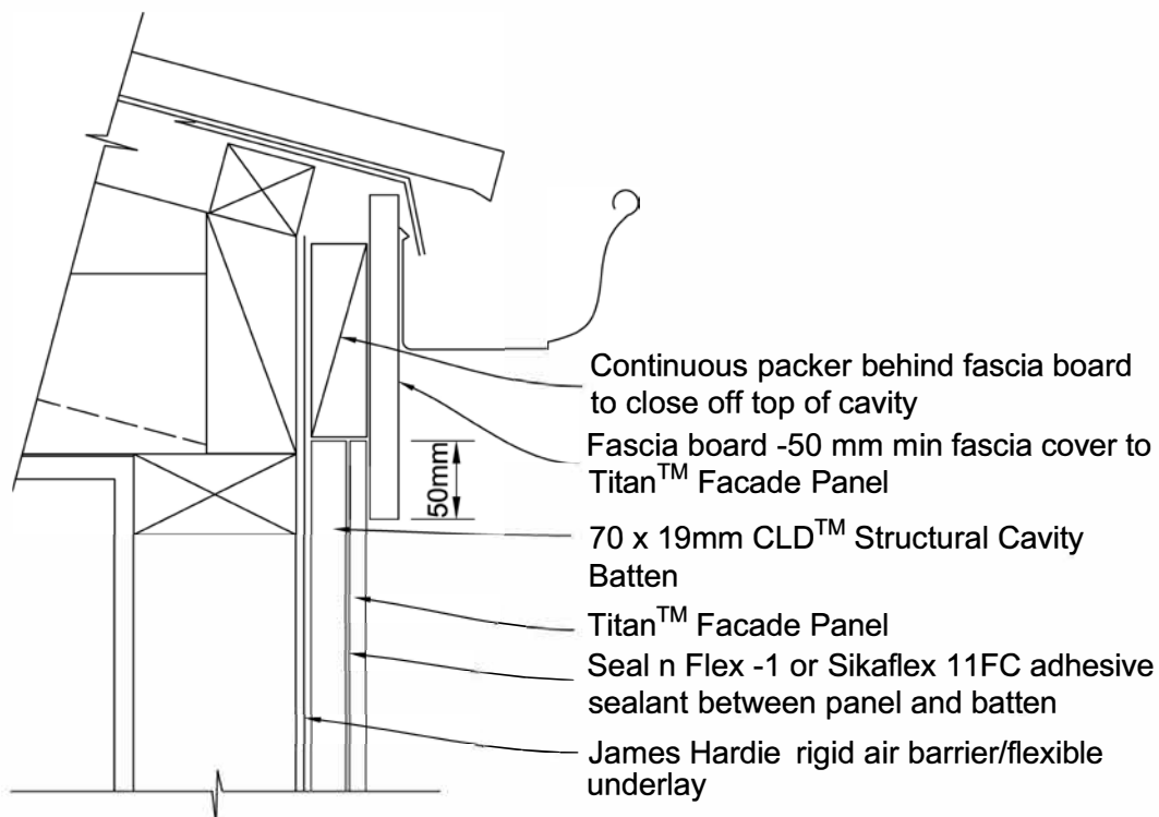
Figure 21: Nil soffit
