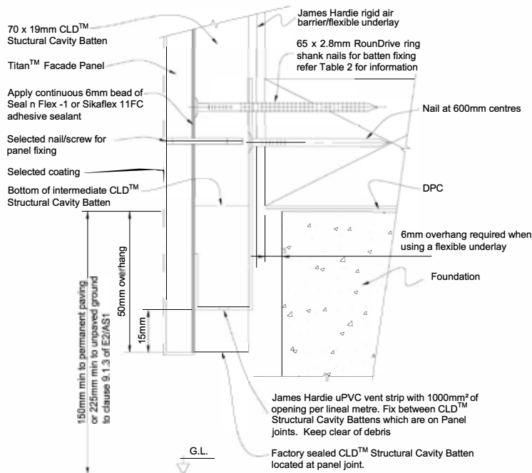
Figure 5: Foundation detail
