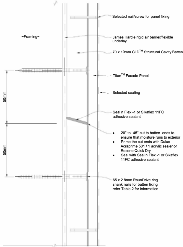
Figure 16: Jointing of CLD Structural Cavity Batten
