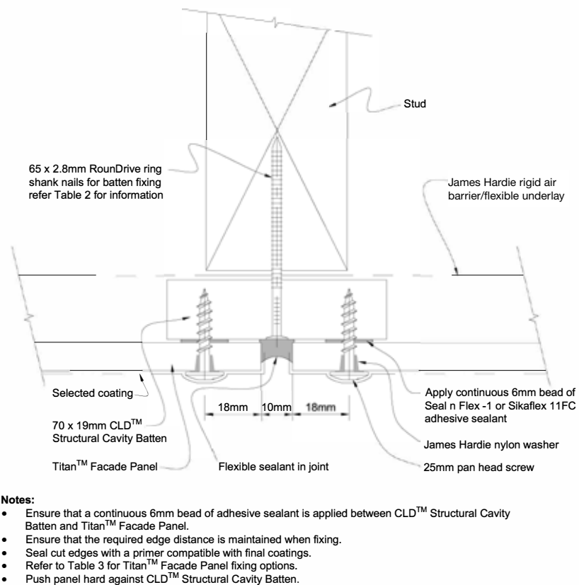
Figure 12: Alternate vertical expressed joint using exposed screws
