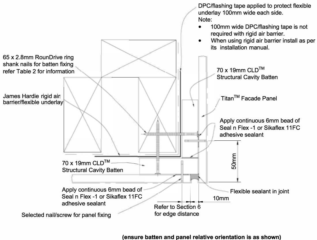
Figure 14: External corner
