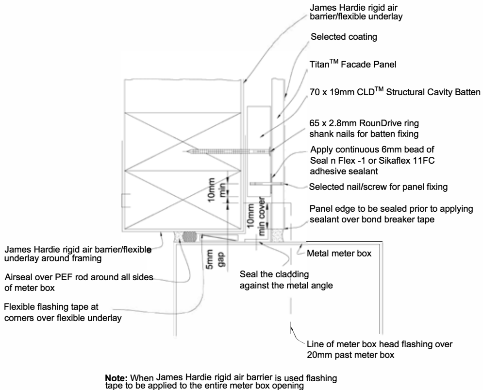
Figure 31: Meter box at jamb
