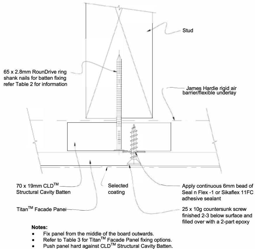
Figure 11: Alternate intermediate stud fixing using countersunk screws
