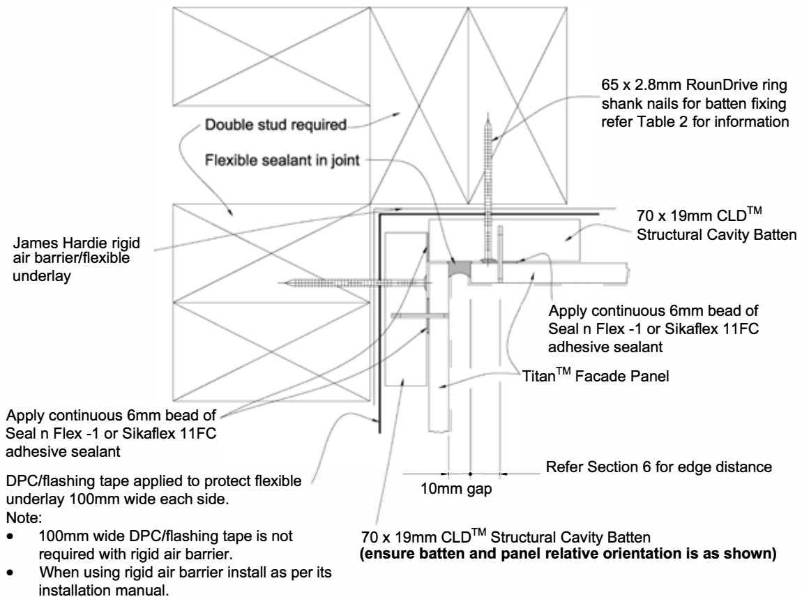
Figure 13: Internal corner
