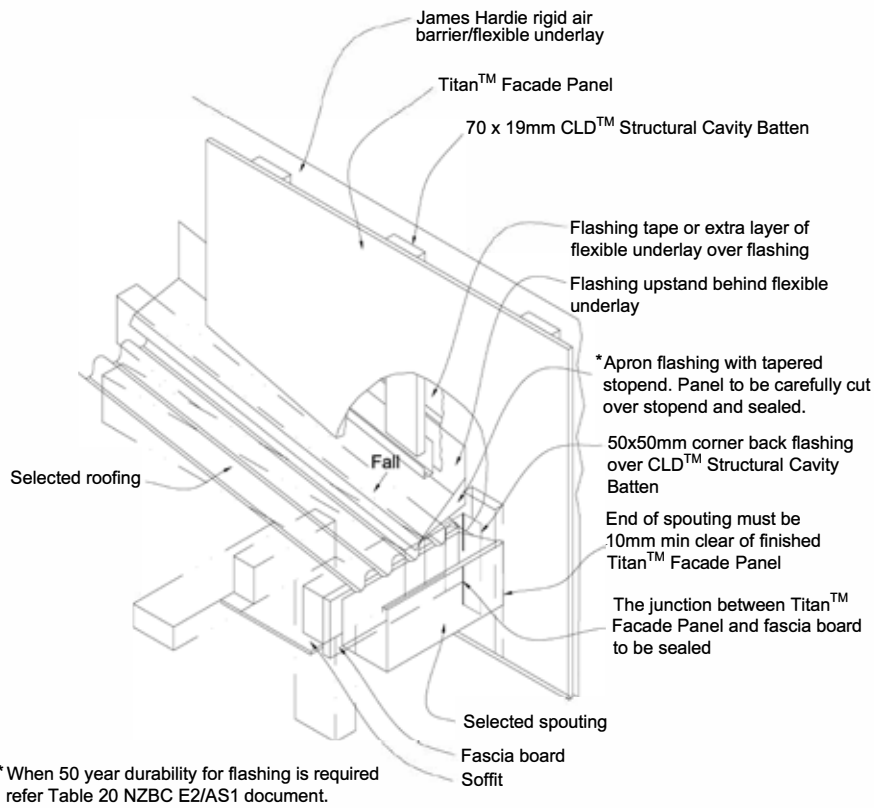
Figure 28: Roof to wall junction detail
