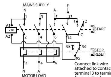
Single Phase & Neutral Supply – 56MS230
