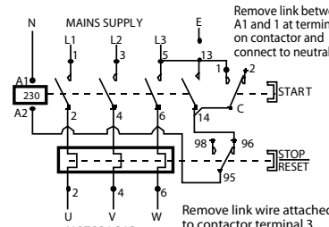
3 Phase 4 Wire Supply – 56MS230
