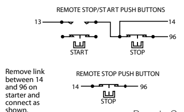
Remote Controls
