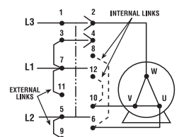
Three Phase Reversing
