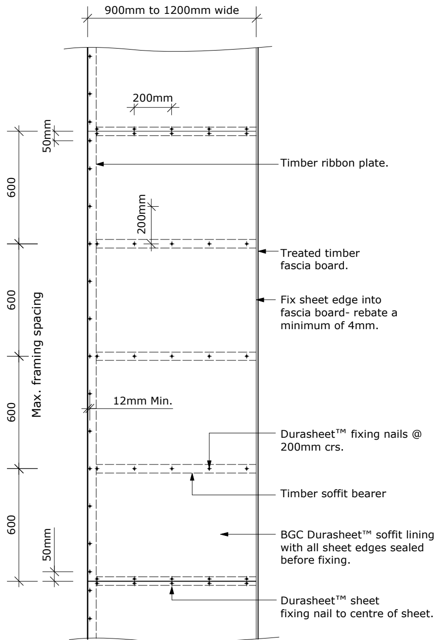
BGC Durasheet™ 900mm to 1200mm Wide Soffit & Eaves Setout
