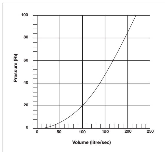
Performance - DCT0708/DCT0709
